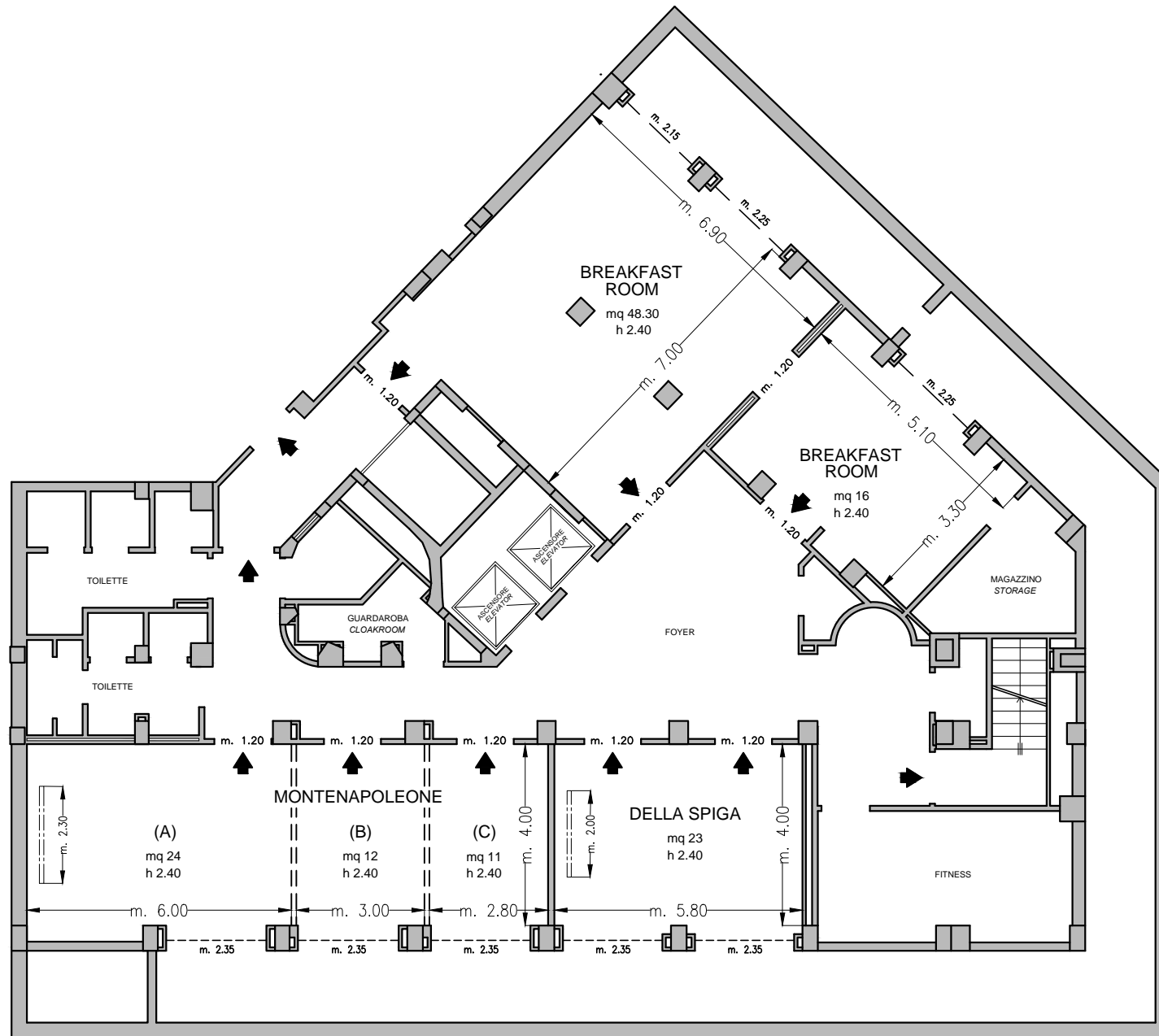
Piano -1 / Basement
